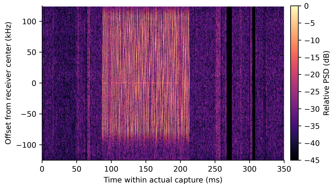
C Real SF8 packet · CRC b746
