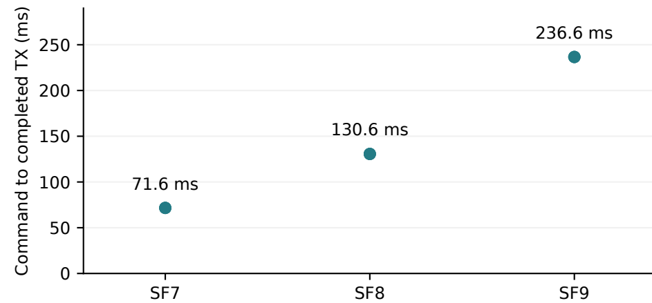
B Actual chip completion, 32 bytes / CR4/8
