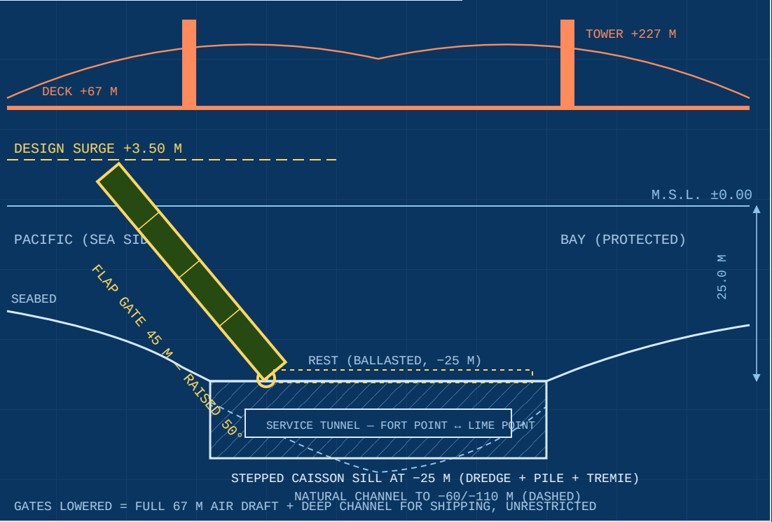
SECTION A-A – BARRIER + BRIDGE
