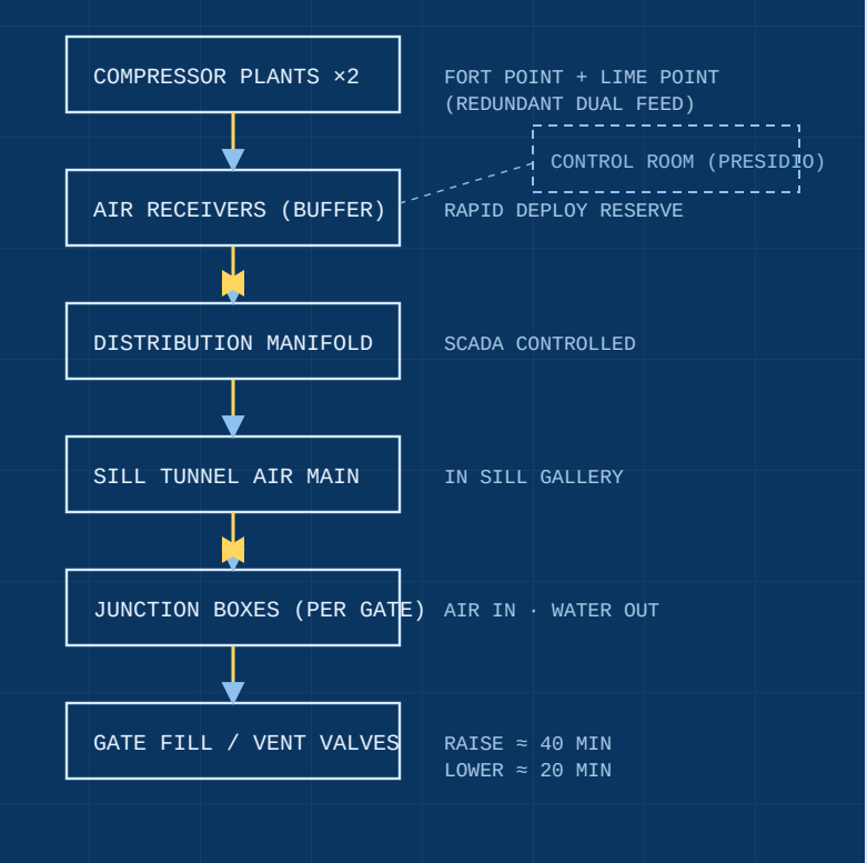
PNEUMATIC + POWER SCHEMATIC
