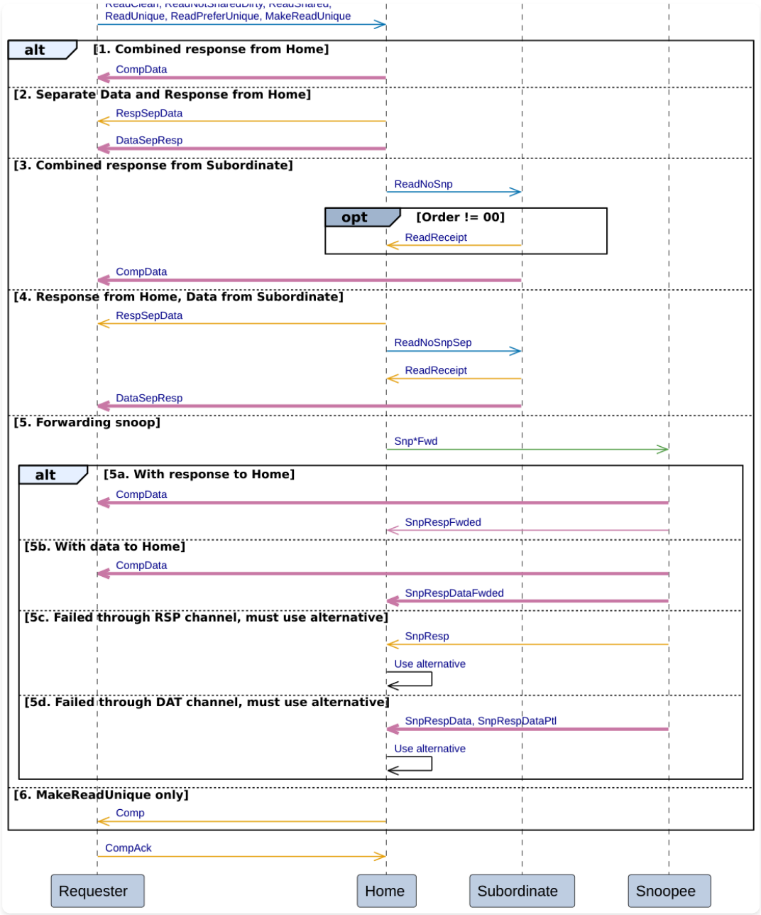
Figure p56 图 B2.1: Allocating Read
