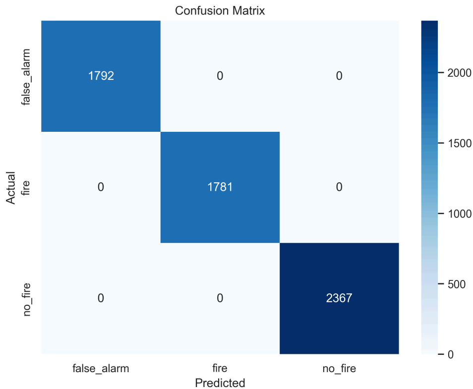
Figure 16: Model Confusion Matrix. A matrix visualizing the predicted vs. actual class labels.
