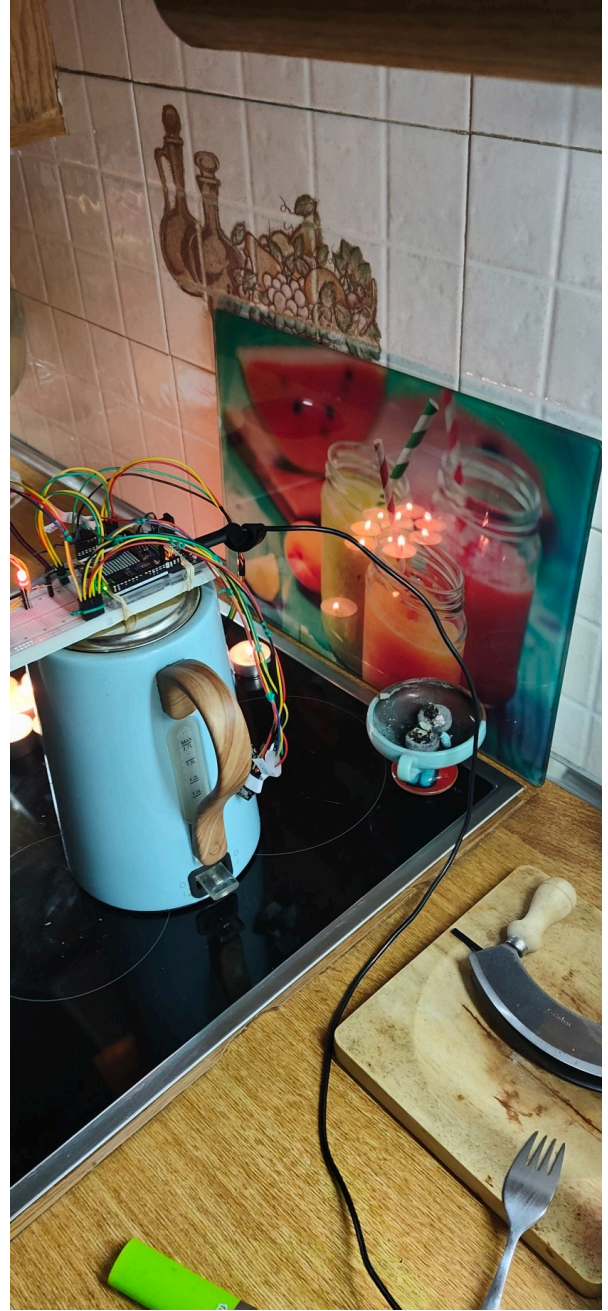
Figure 2: Indoor Fire Data Collection. Left: capturing infrared signatures from a flame source; Right: capturing combined flame and smoke signatures.
