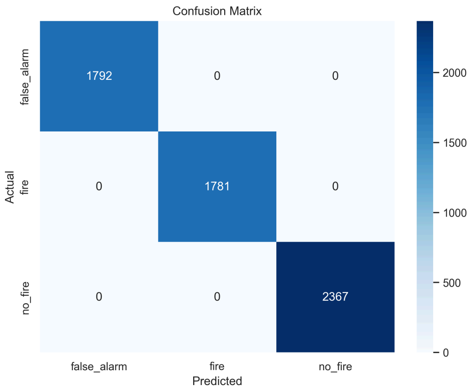
Figure 16: Model Confusion Matrix. A matrix visualizing the predicted vs. actual class labels. The 100% accuracy in this controlled environment demonstrates the high mathematical separability of the fire and false alarm classes under ideal conditions.
