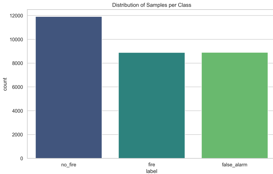
Figure 17: Dataset Class Distribution. A bar chart representing the number of samples for each of the three target classes: fire, no_fire, and false_alarm. The distribution confirms a well-balanced dataset, preventing model bias.
