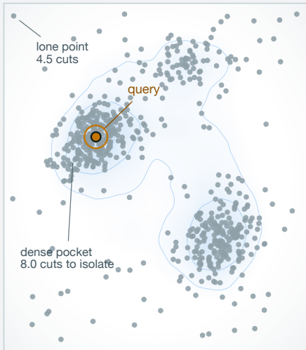
a Dense pockets resist isolation
