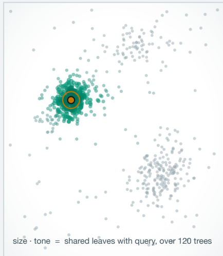
c Many trees: leafmates assemble
