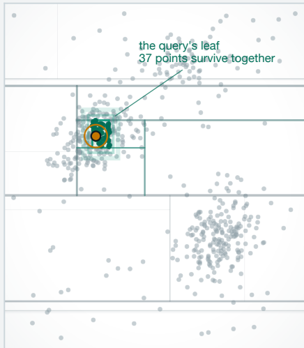
b One tree: the cuts that failed
