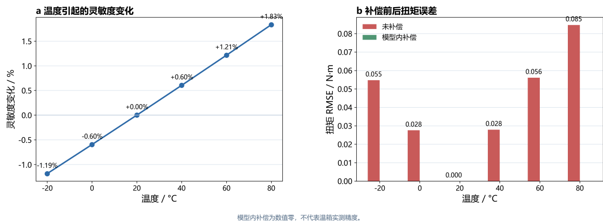
图 8 温度引起的灵敏度变化及模型逆变换误差 Fig.8 Temperature-induced sensitivity variation and model-inversion error
