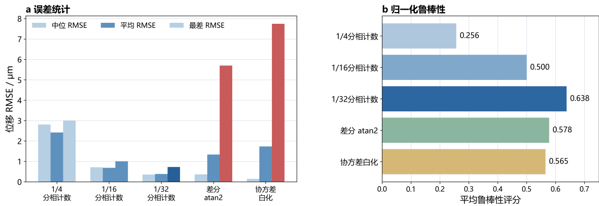
图 7 五种解调算法的误差统计与归一化鲁棒性 Fig.7 Error statistics and normalized robustness of five demodulation algorithms
