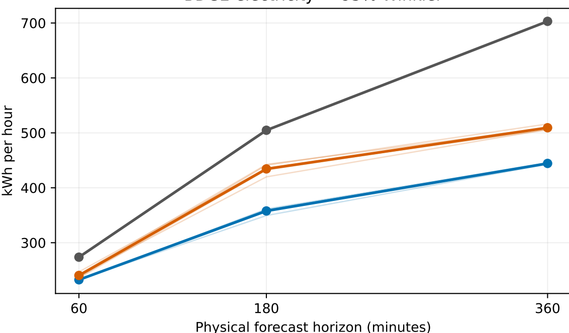
BDG2 electricity — 95% Winkler
