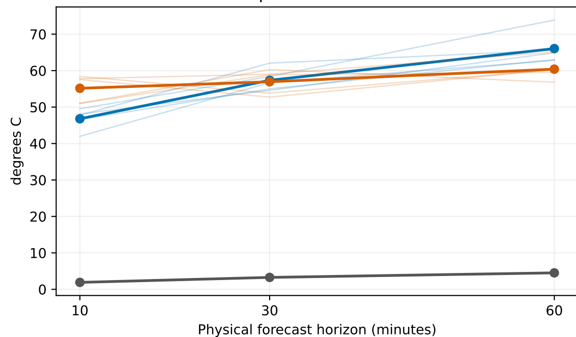
PLEIA energy — 95% Winkler
