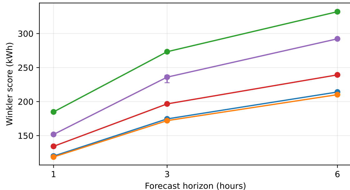
90% intervals
