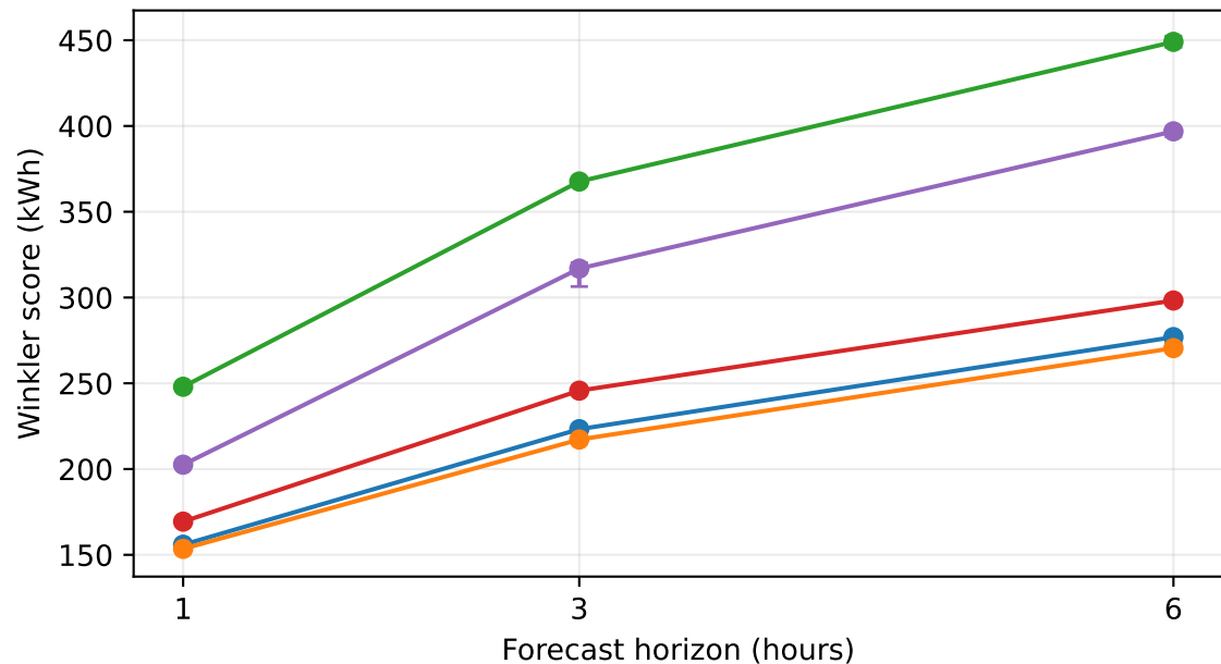
95% intervals
