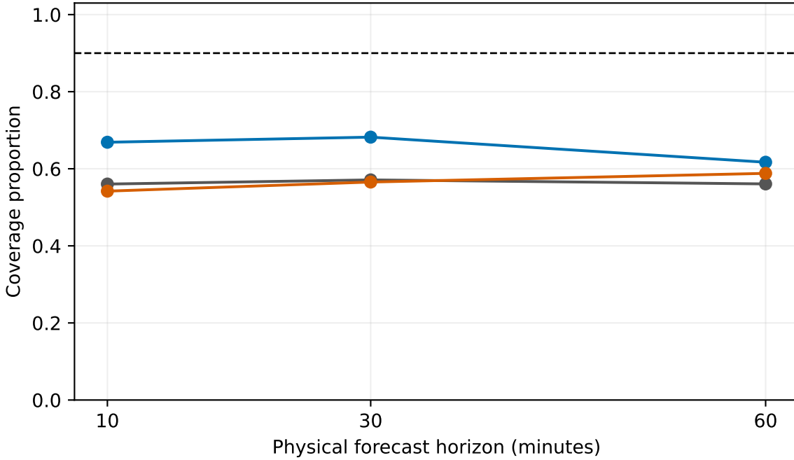
RICO temperature — 90% interval coverage
