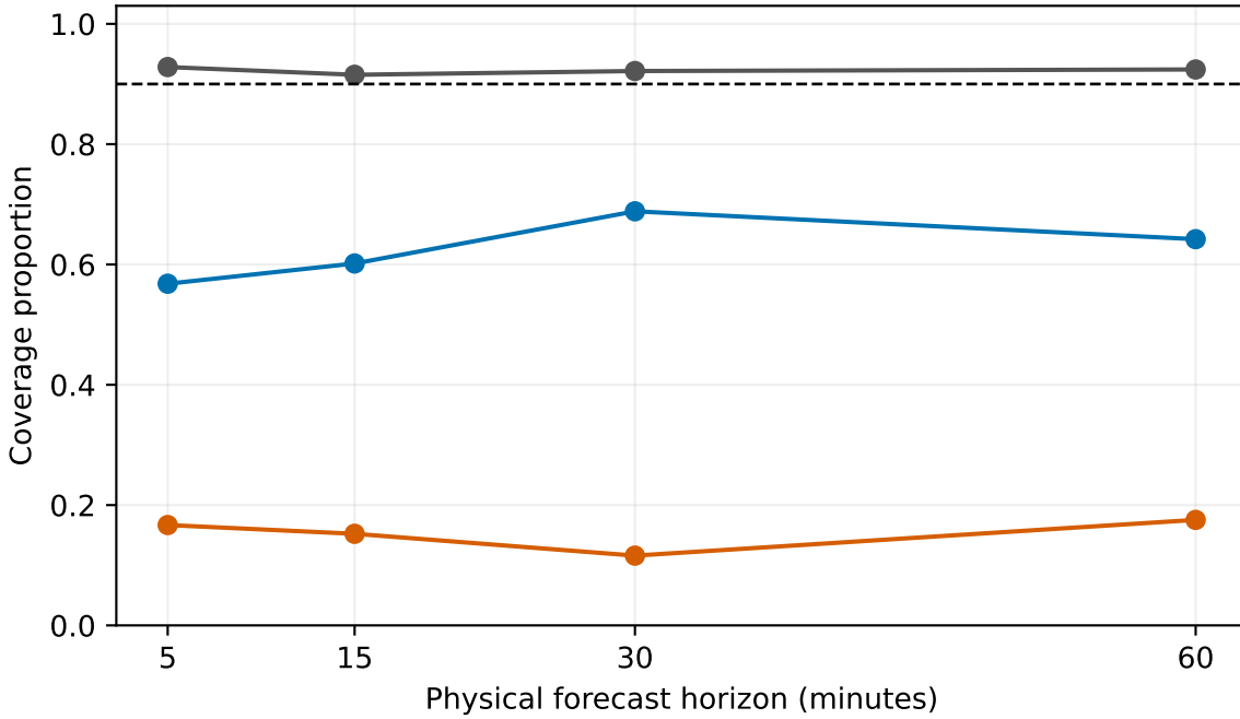
BDG2 electricity — 90% interval coverage
