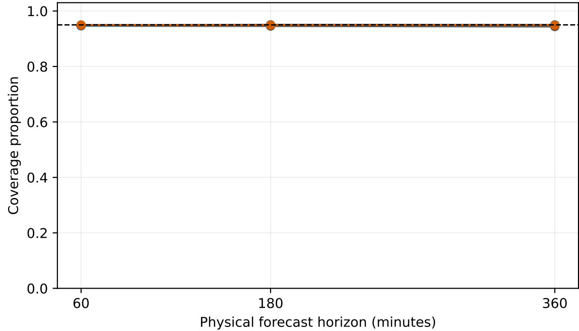
BDG2 electricity — 95% interval coverage
