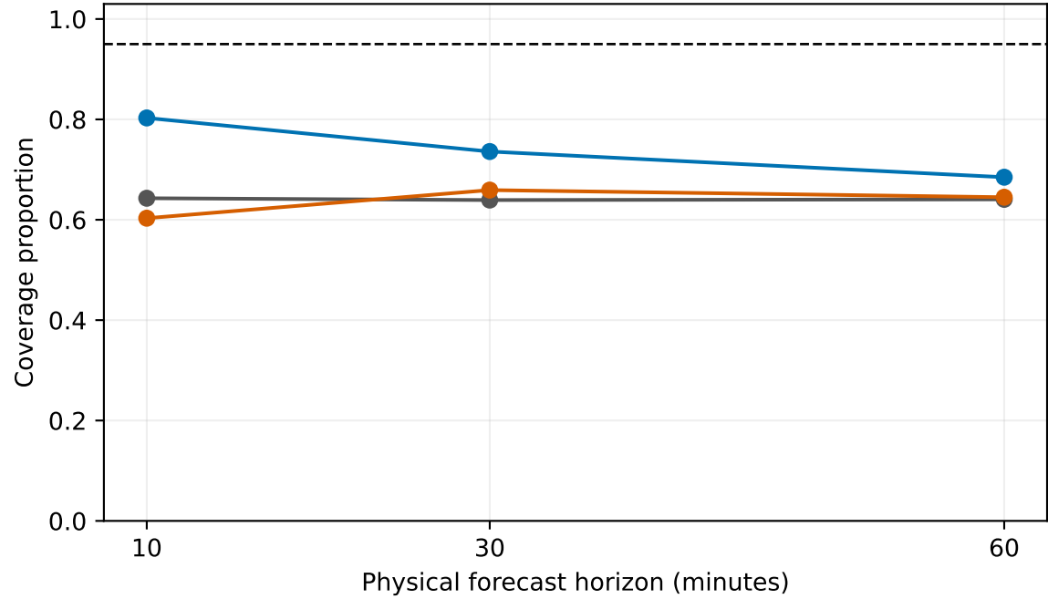
RICO temperature — 95% interval coverage
