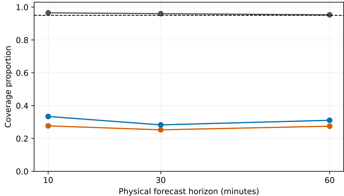
PLEIA energy — 95% interval coverage
