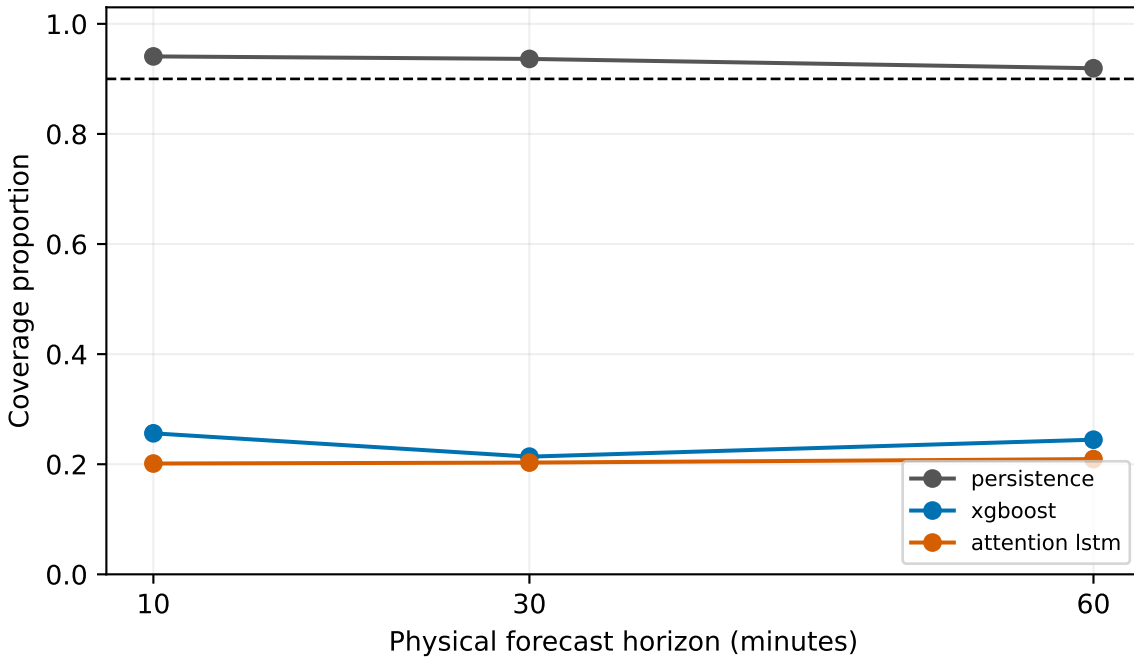
PLEIA energy — 90% interval coverage
