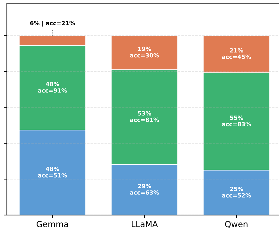
ProofWriter
