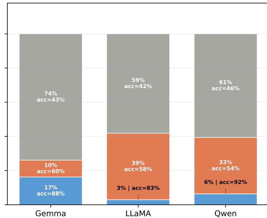
FOLIO
