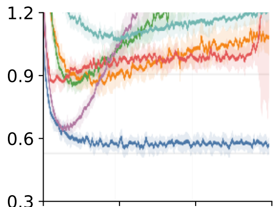
Validation loss
