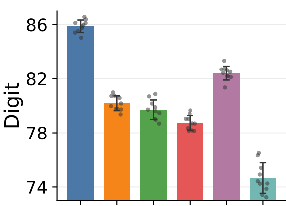
Test accuracy
