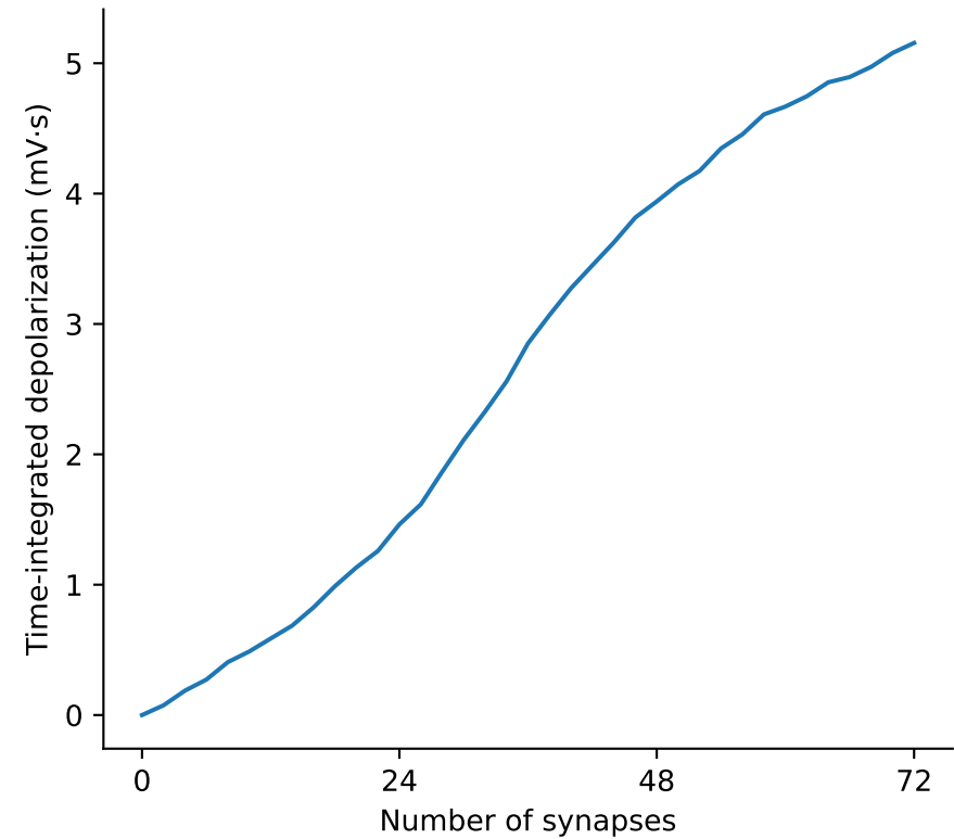
Integrated depolarization vs synaptic activation
