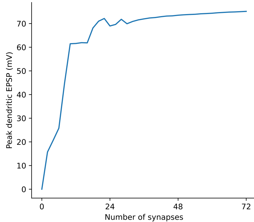
Dendritic EPSP peak vs synaptic activation
