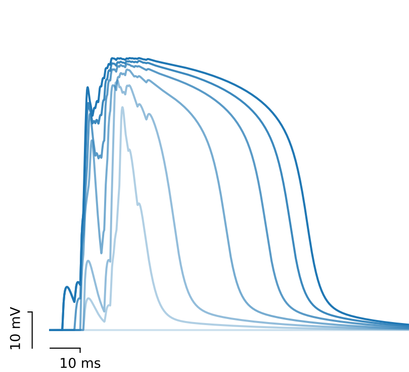
Dendritic EPSPs across activation levels
