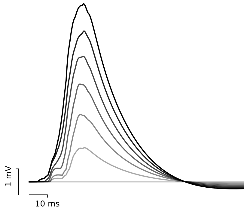
Soma EPSPs (expected)
