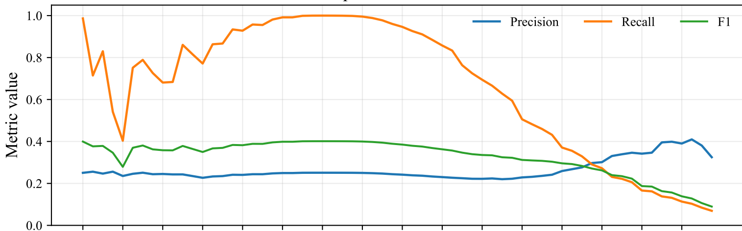
amazon: precision/recall at L=20
