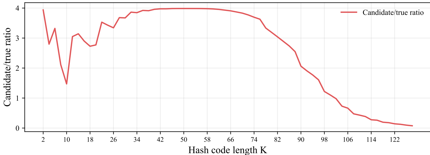
amazon: candidate/true ratio at L=20
