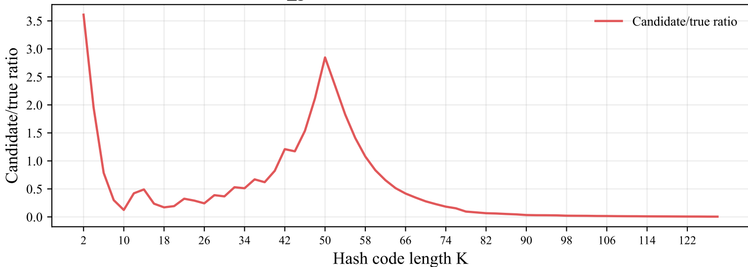
cifar10_gist512: candidate/true ratio at L=20
