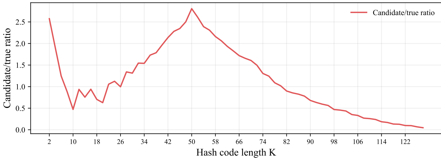
isolet: candidate/true ratio at L=20
