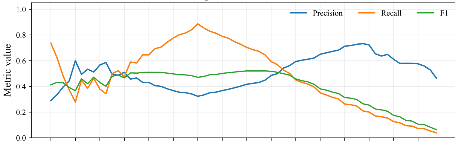
isolet: precision/recall at L=20
