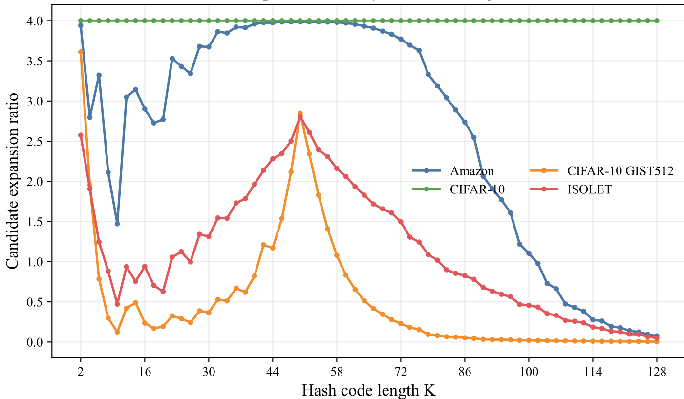
Candidate expansion ratio by hash code length at L=20
