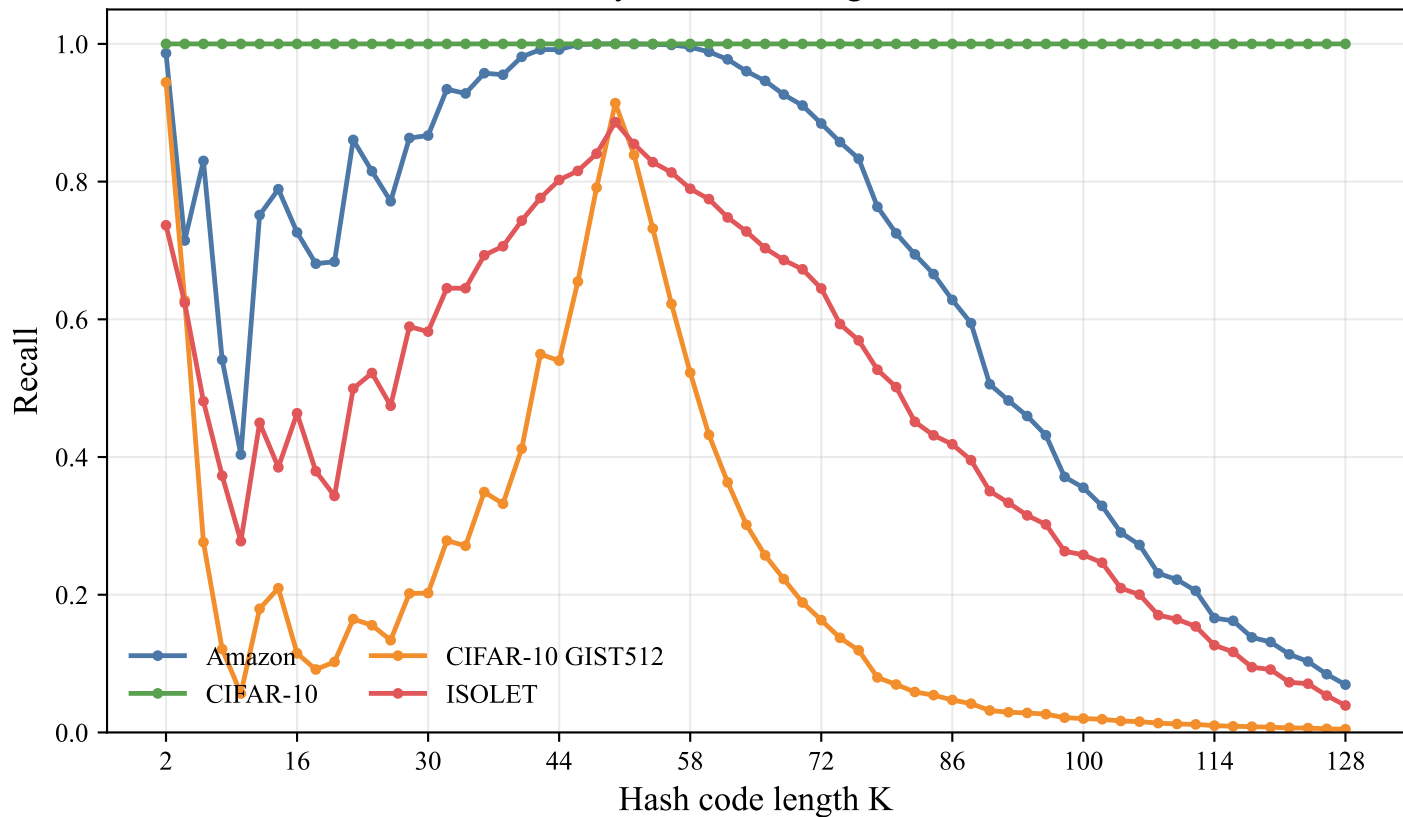
Recall by hash code length at L=20
