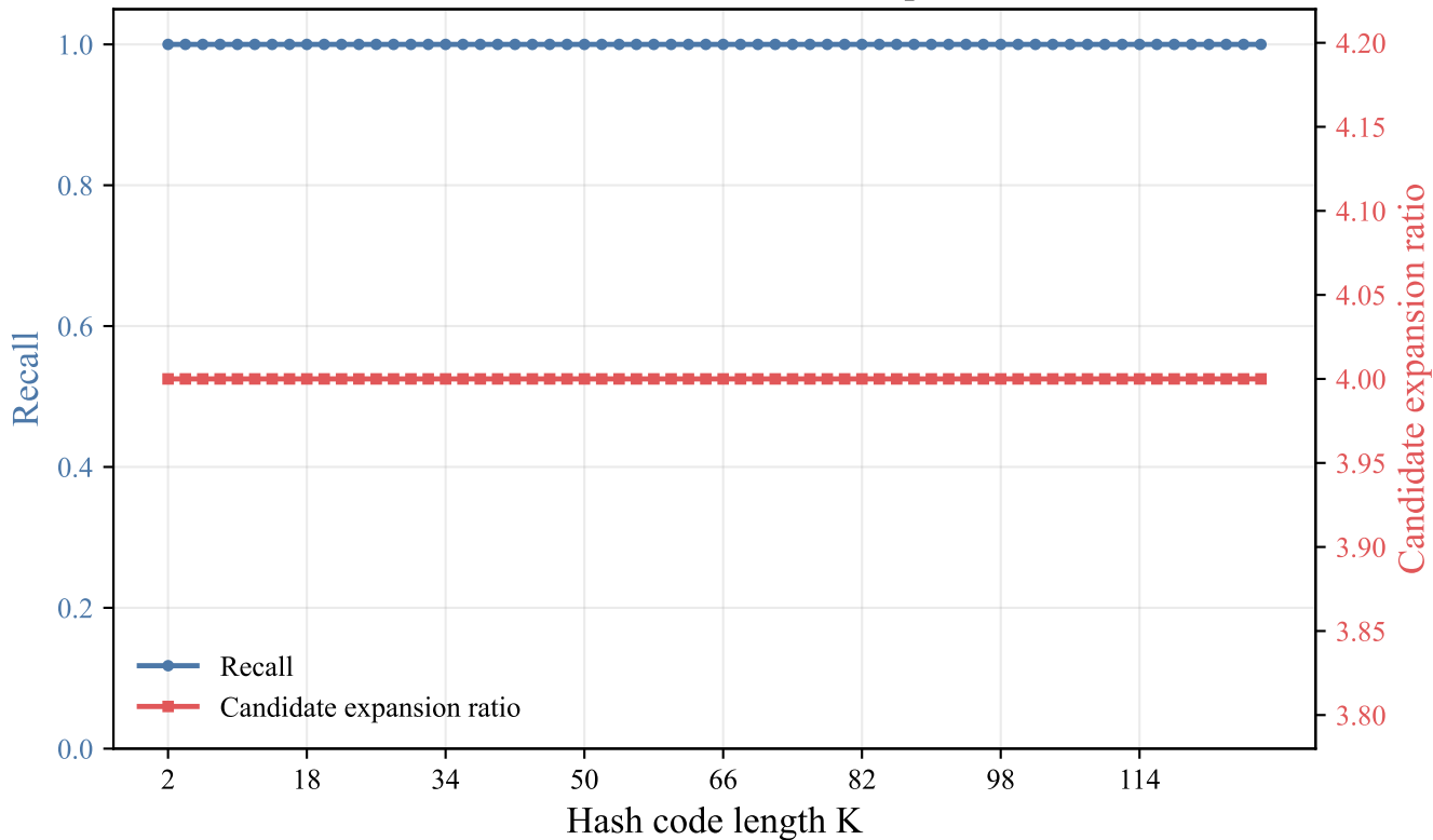
cifar10: recall and candidate expansion
