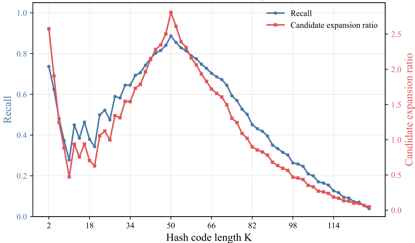
isolet: recall and candidate expansion
