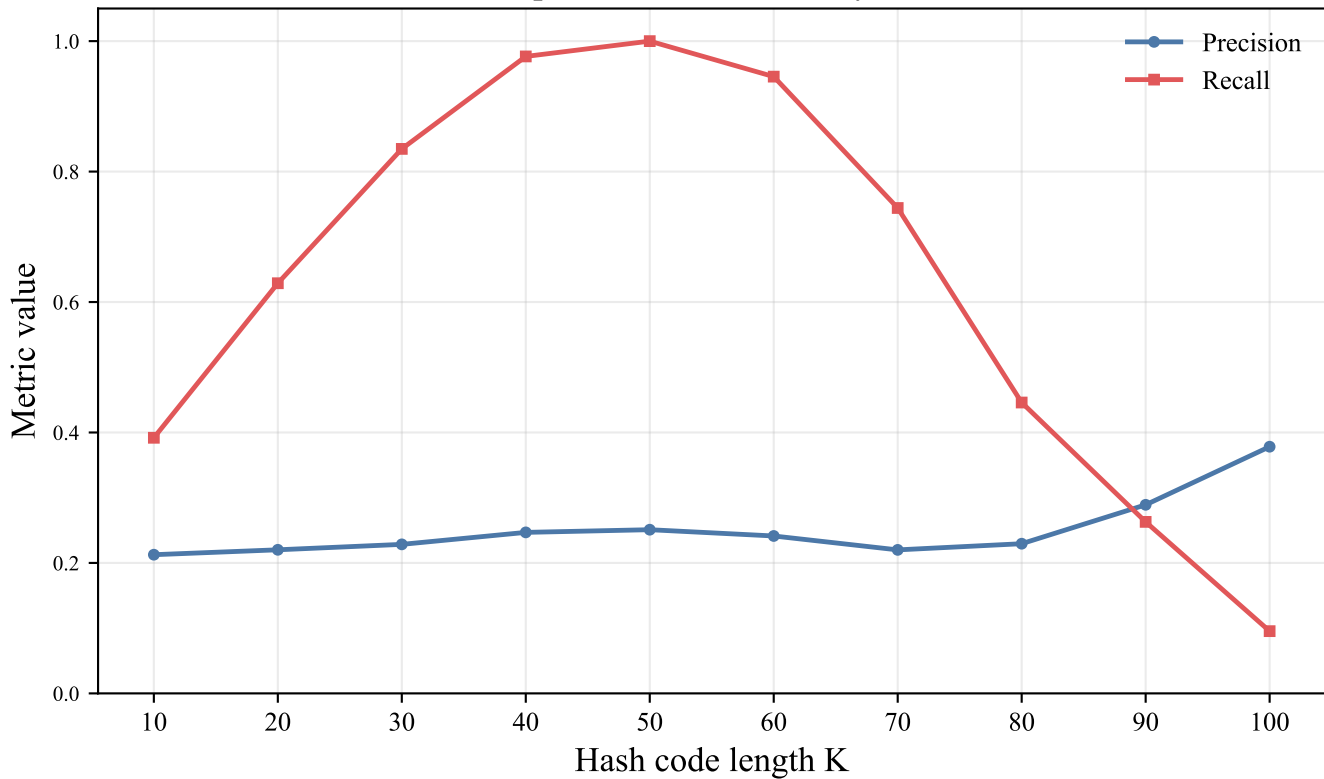
Amazon: precision and recall by K at L=20
