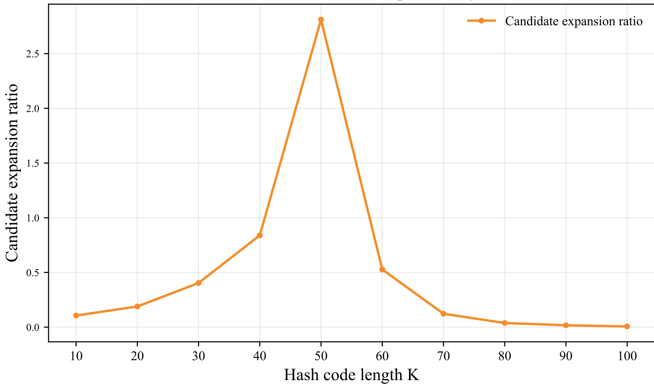
CIFAR-10 GIST512: candidate expansion by K at L=20
