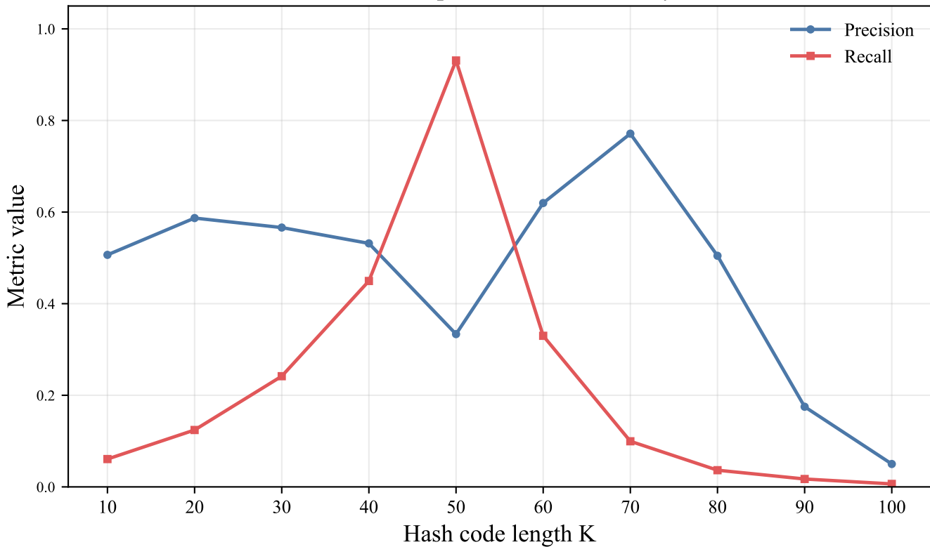
CIFAR-10 GIST512: precision and recall by K at L=20
