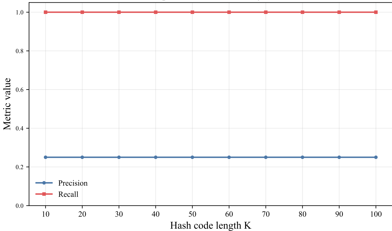
CIFAR-10: precision and recall by K at L=20
