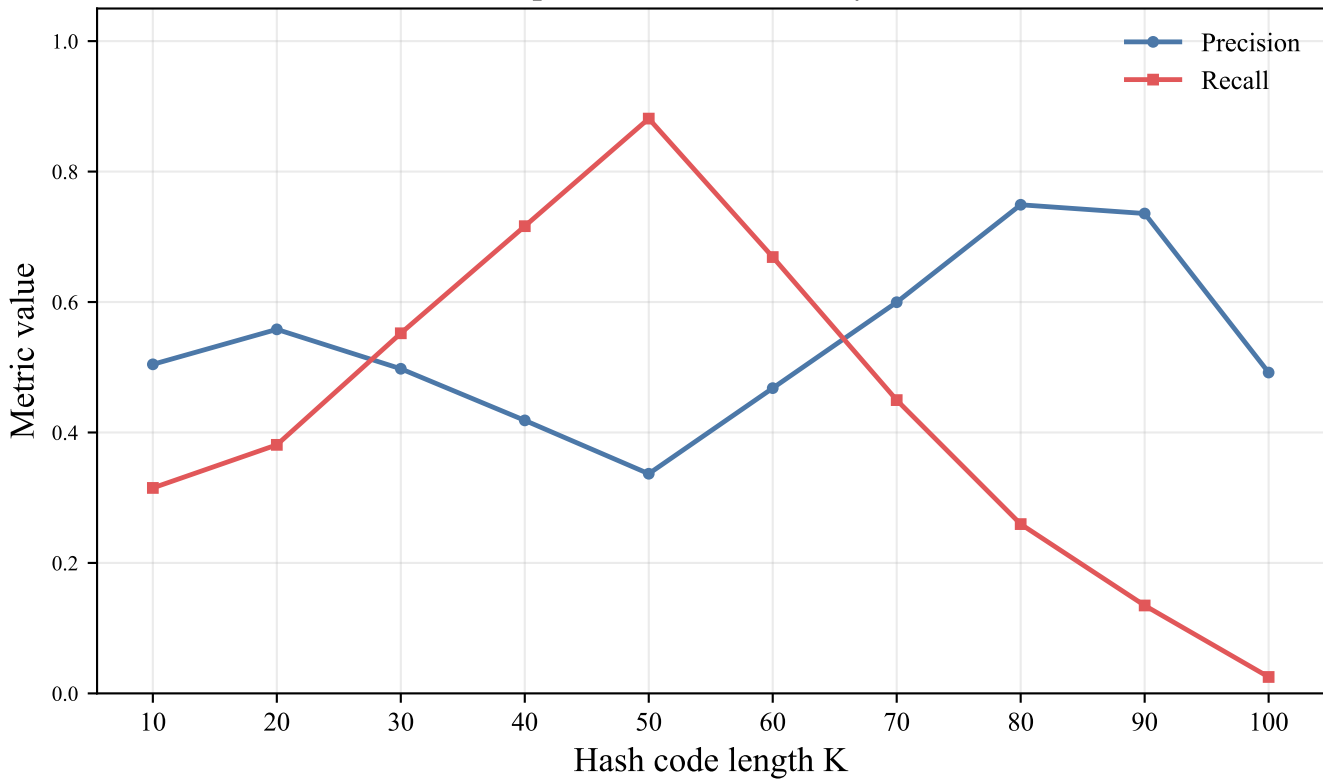
ISOLET: precision and recall by K at L=20
