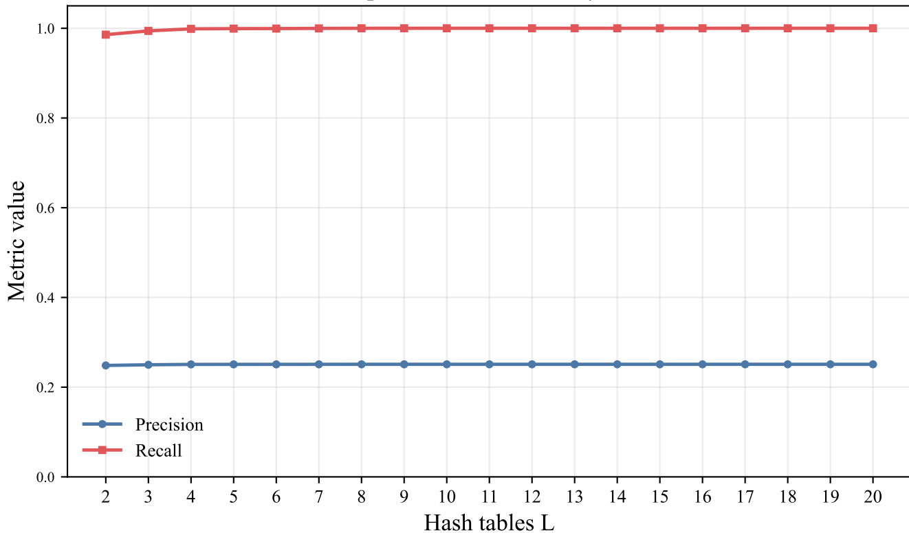
Amazon: precision and recall by L at K=50
