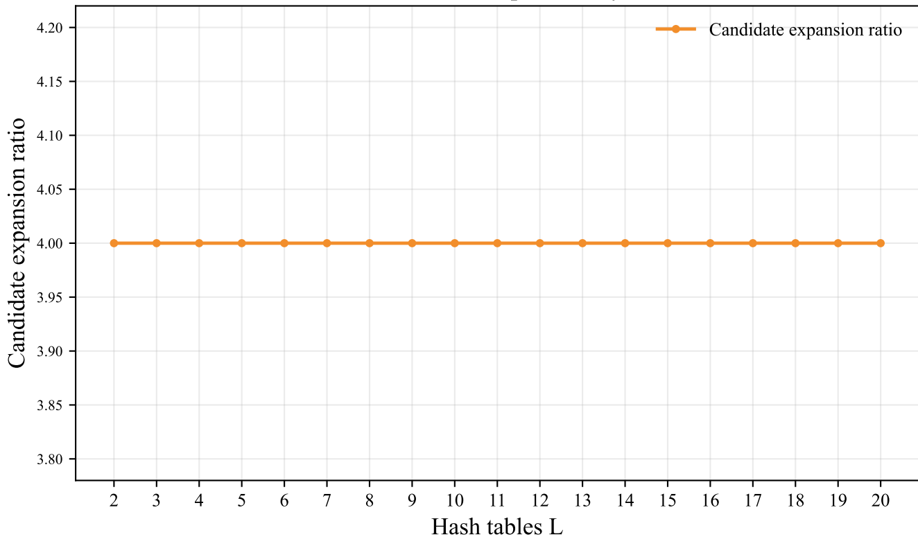
CIFAR-10: candidate expansion by L at K=50
