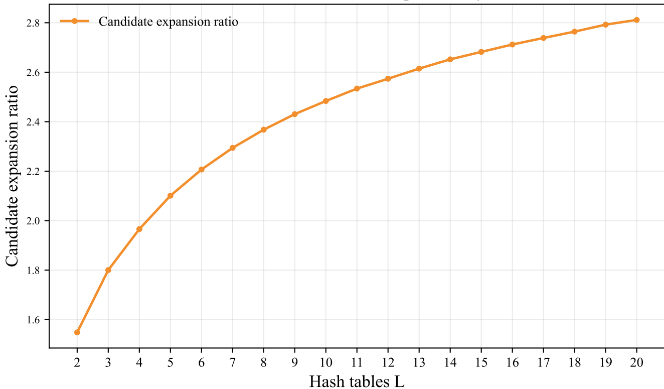
CIFAR-10 GIST512: candidate expansion by L at K=50
