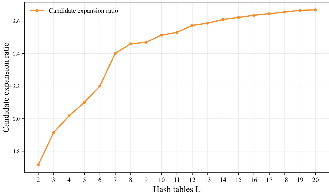
ISOLET: candidate expansion by L at K=50
