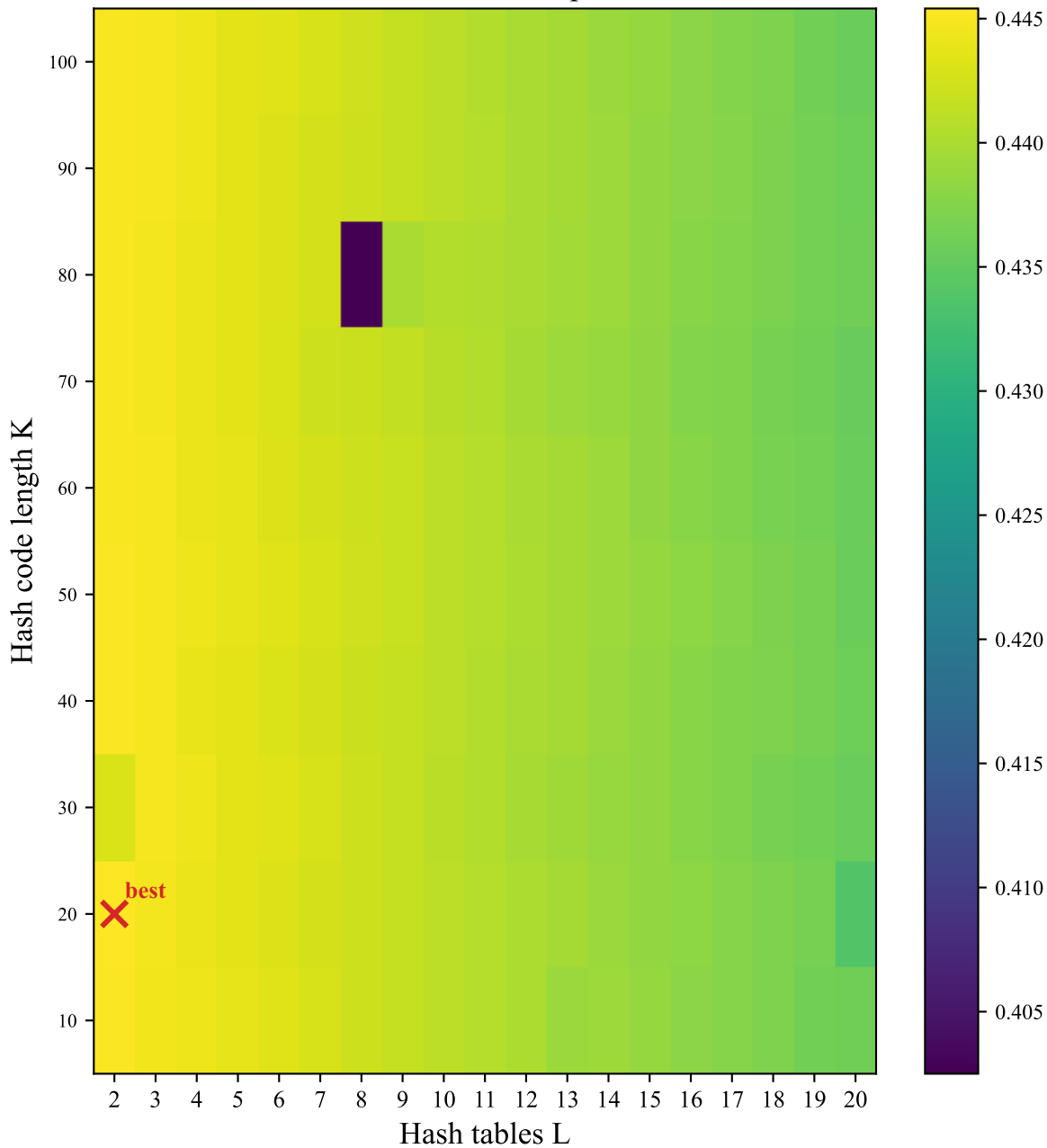
cifar10: Recall-constrained precision score
