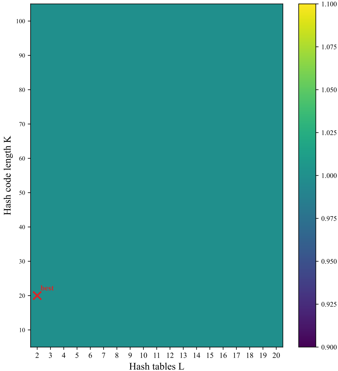
cifar10: Recall
