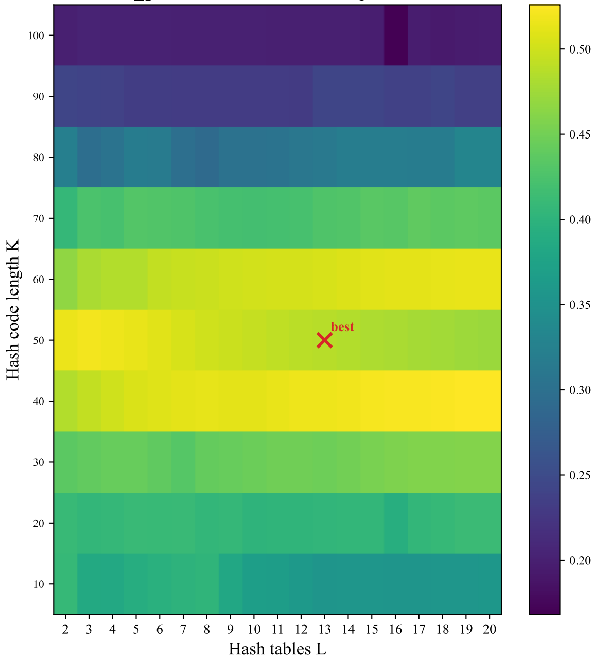
cifar10_gist512: Recall-constrained precision score
