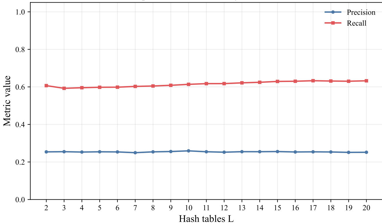
Amazon: precision and recall by hash table count
