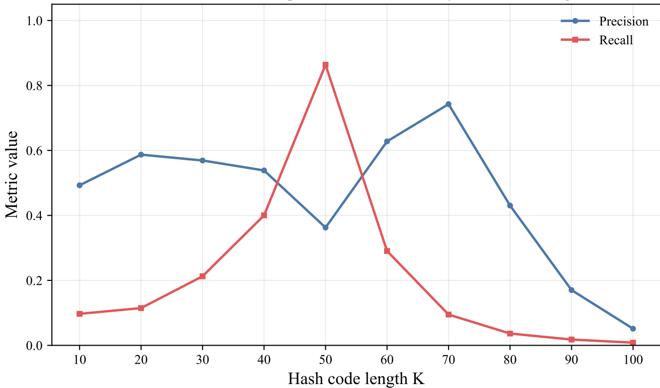
CIFAR-10 GIST512: precision and recall by hash code length
