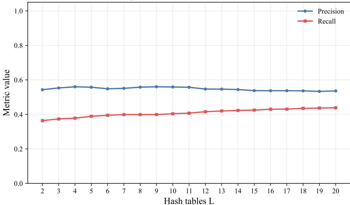
ISOLET: precision and recall by hash table count
