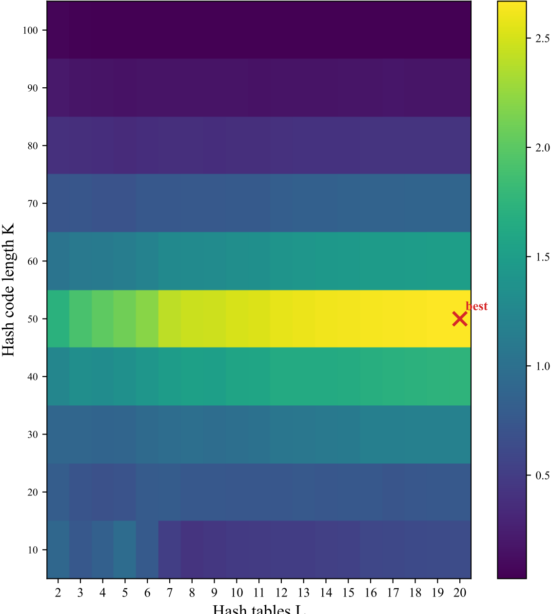
isolet: Candidate expansion ratio
