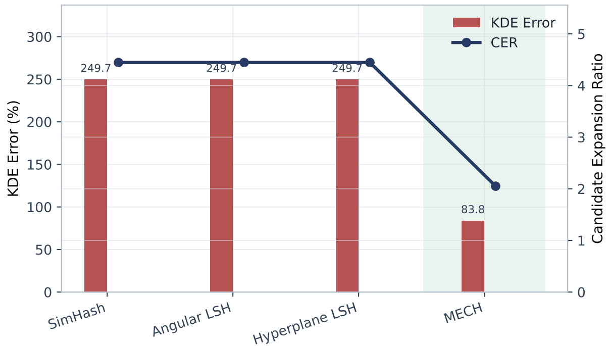
KDE Error and Candidate Cost
