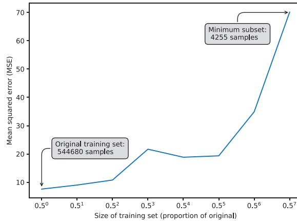
Fig. 7. MSE of the NN model in relation to the size of the training dataset.
