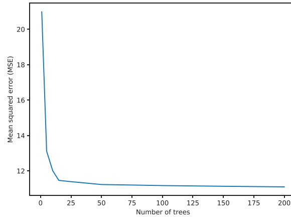
Fig. 4. Results of number of trees test for the RF.
