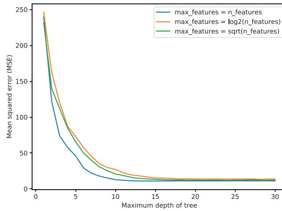
Fig. 5. Results of grid search regarding maximum tree depth and maximum features of the RF.
