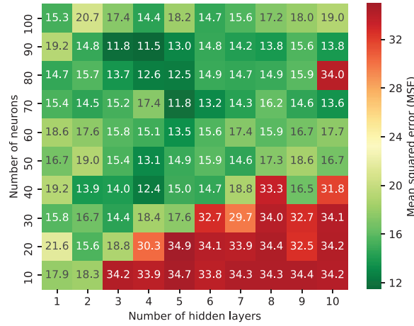
Fig. 2. Results of grid search regarding number of neurons and number of hidden layers of the NN.
