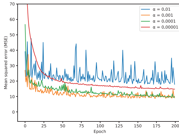
Fig. 3. Results of learning rate testing for the NN.
