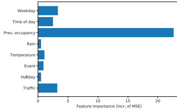
Fig. 8. Results of the performance of the NN model under the feature elimination scenario.
