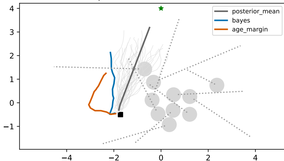
Scene 3, step 24: common candidate evaluation
