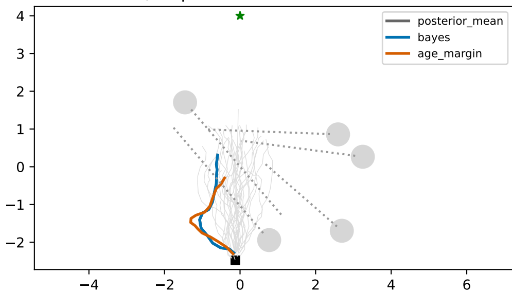
Scene 1, step 8: common candidate evaluation
