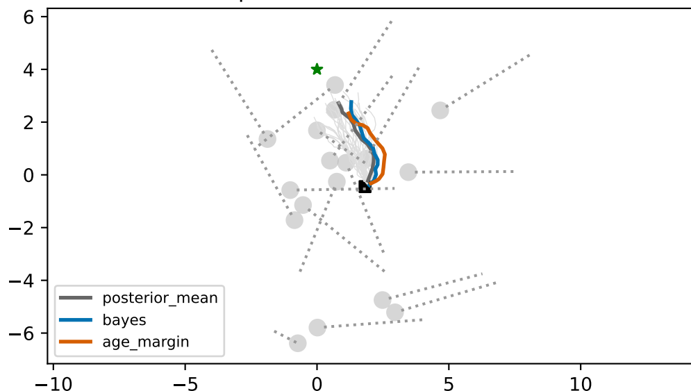
Scene 5, step 24: common candidate evaluation
