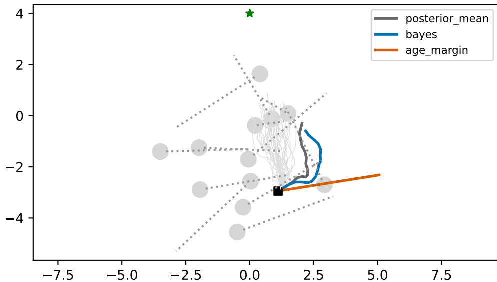
Scene 4, step 8: common candidate evaluation
