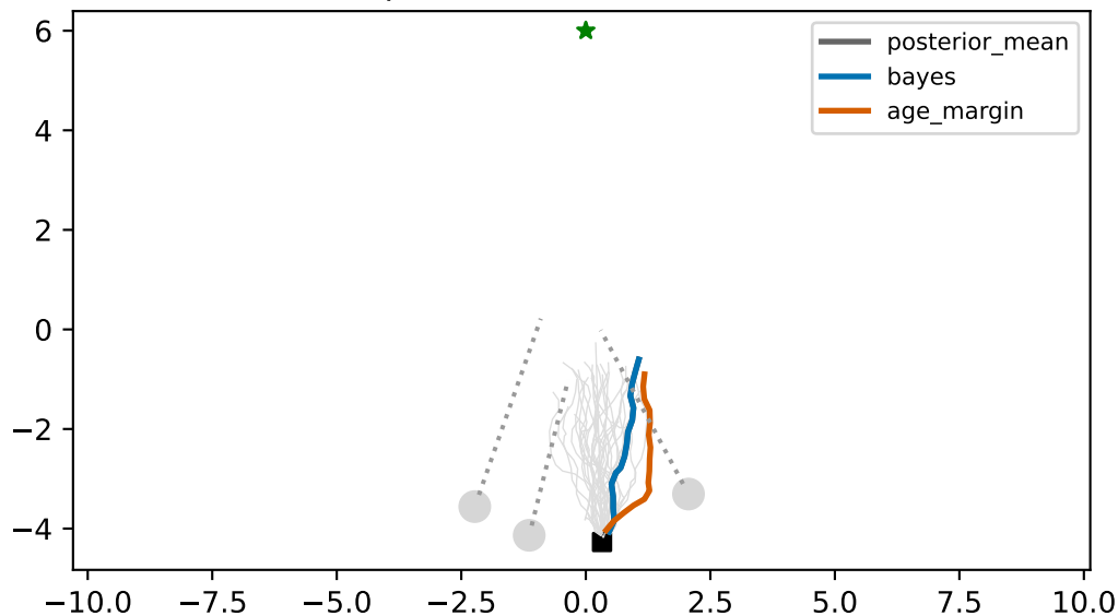
Scene 5, step 8: common candidate evaluation
