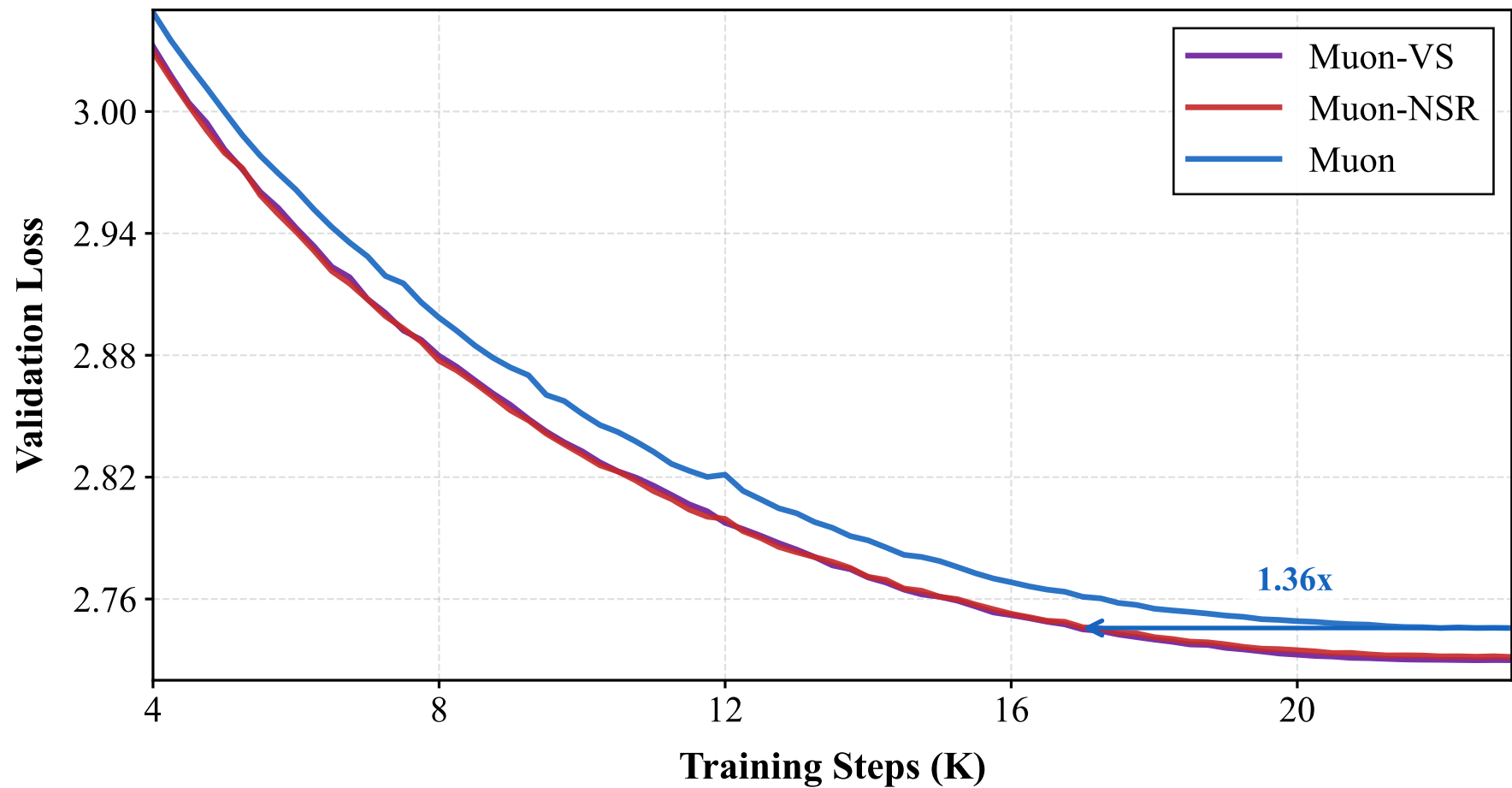
Validation Loss vs Iterations
