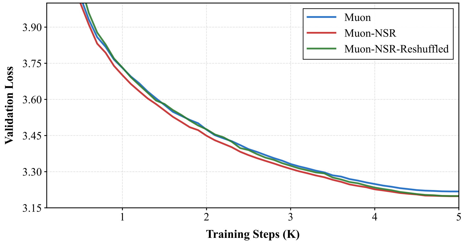
Validation Loss vs Iterations
