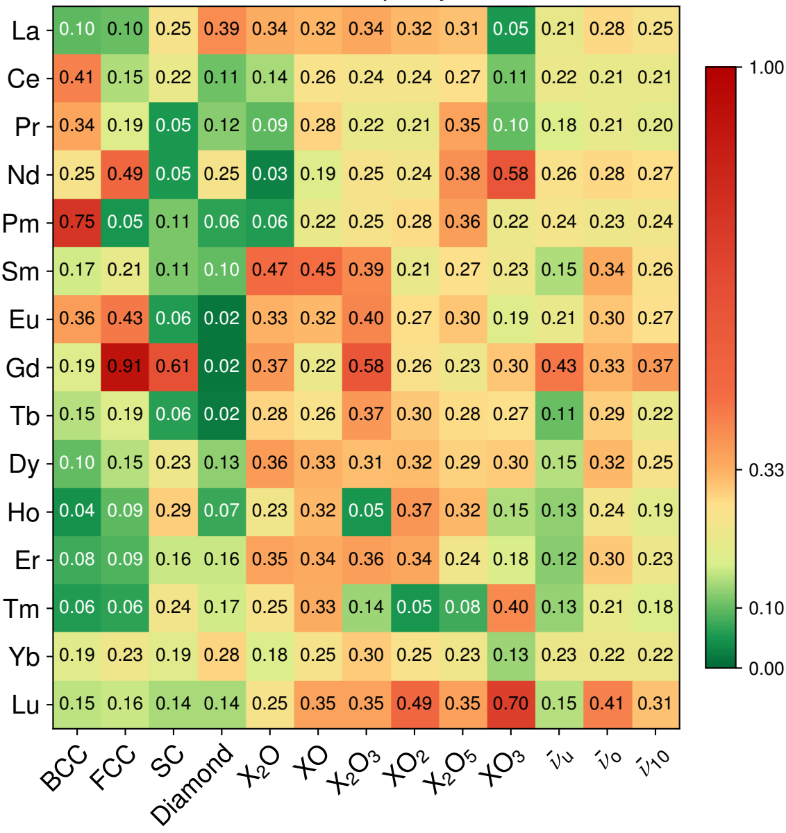
EOS discrepancy: \nu
