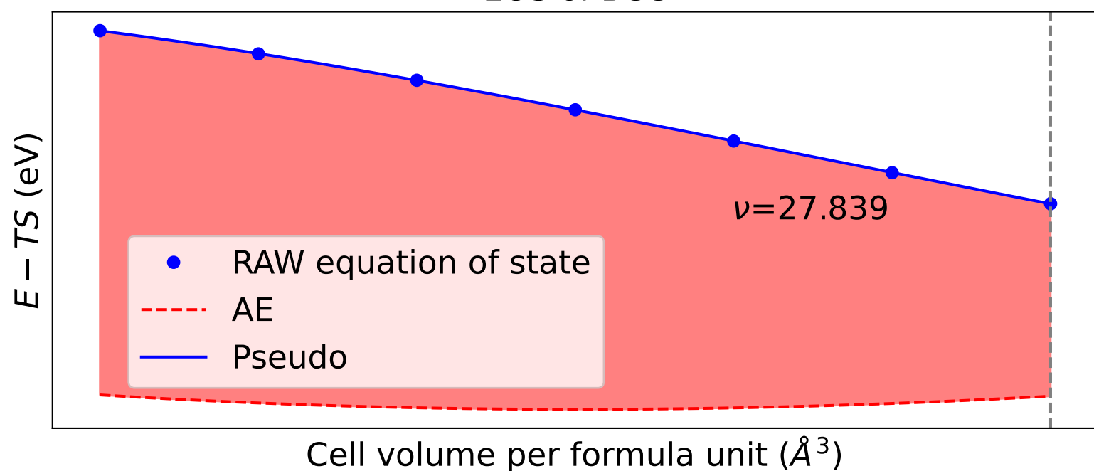
EOS of BCC
