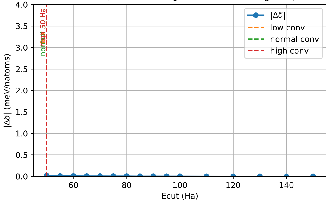
La - FCC (Normalised \Delta_1 difference convergence)
