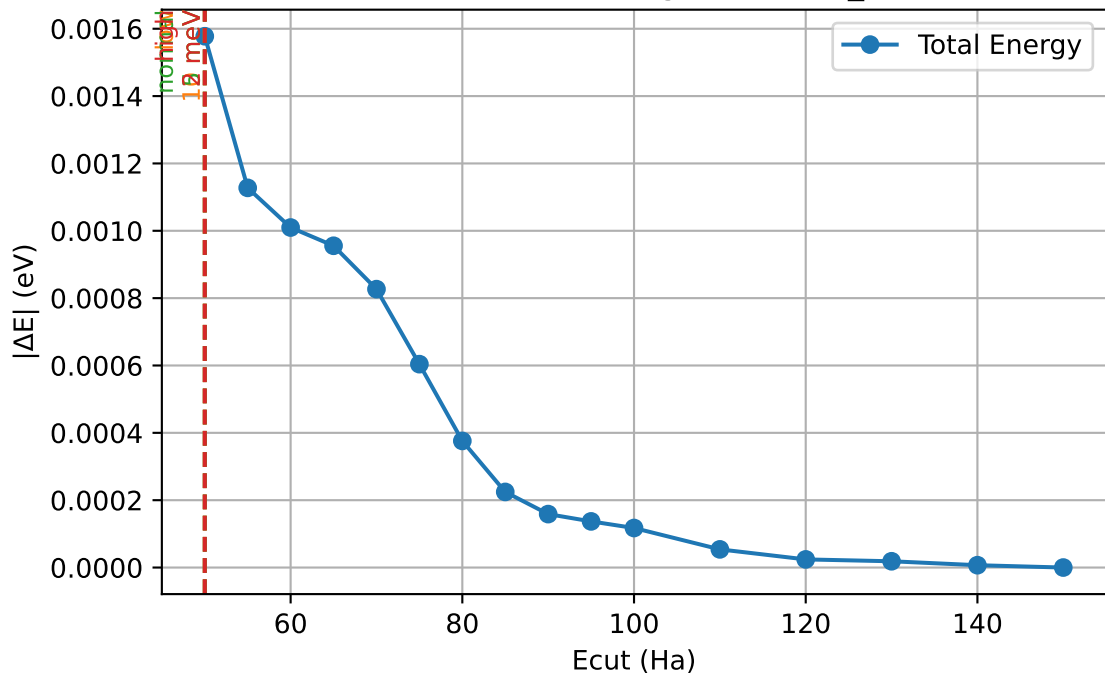
La - FCC (Ecut convergence) [abs_error]
