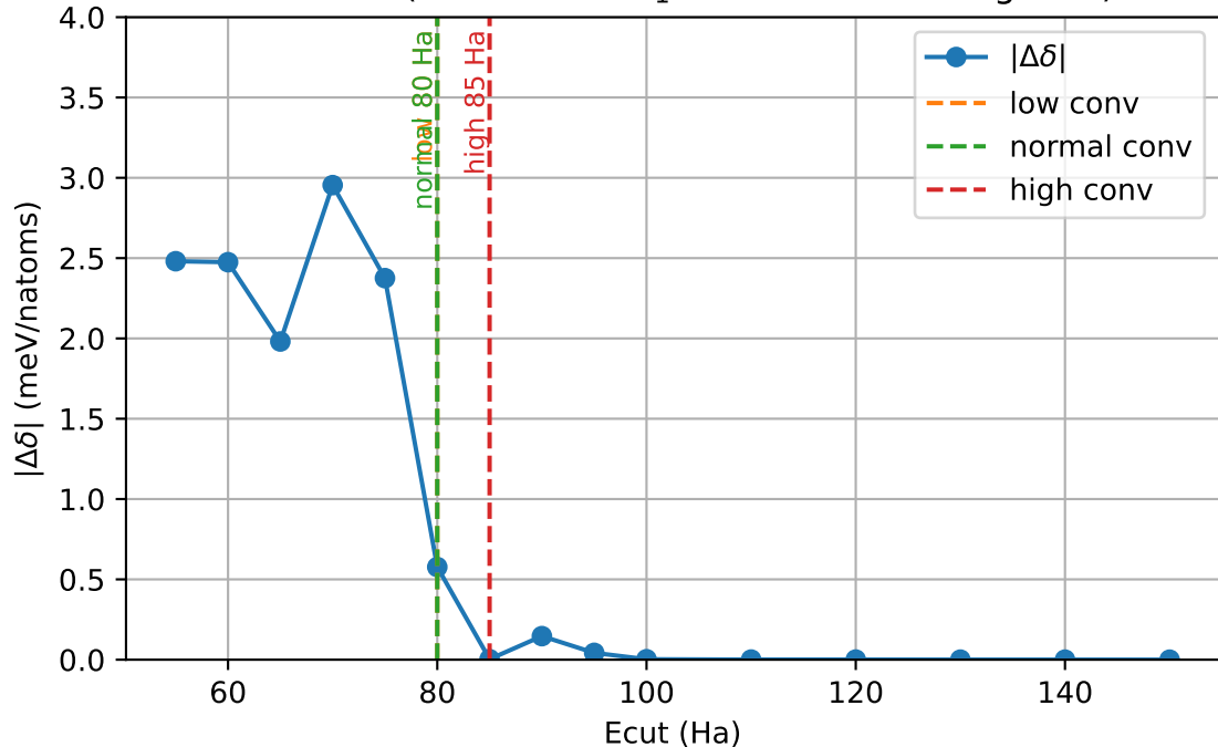
Sm - FCC (Normalised \Delta_1 difference convergence)
