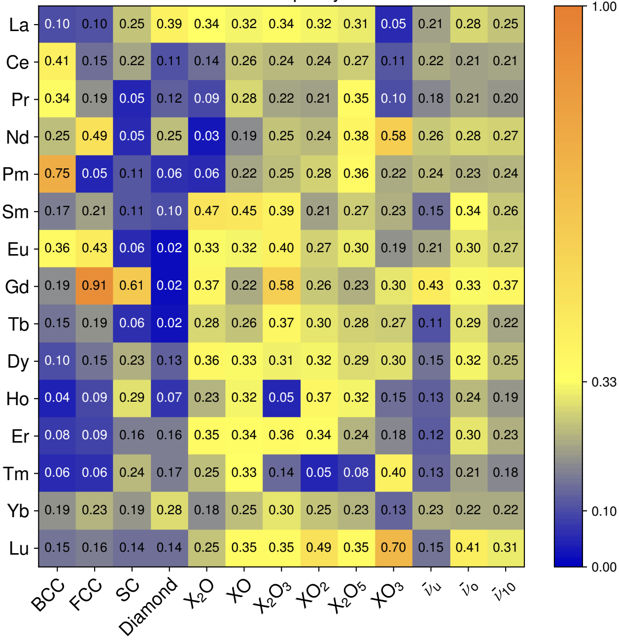
EOS discrepancy: \nu
