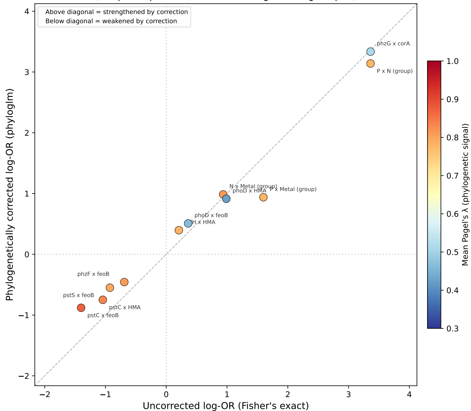
Figure 4. Effect sizes before and after phylogenetic correction (soil/plant species; color = mean Pagel's \lambda of gene pair)
