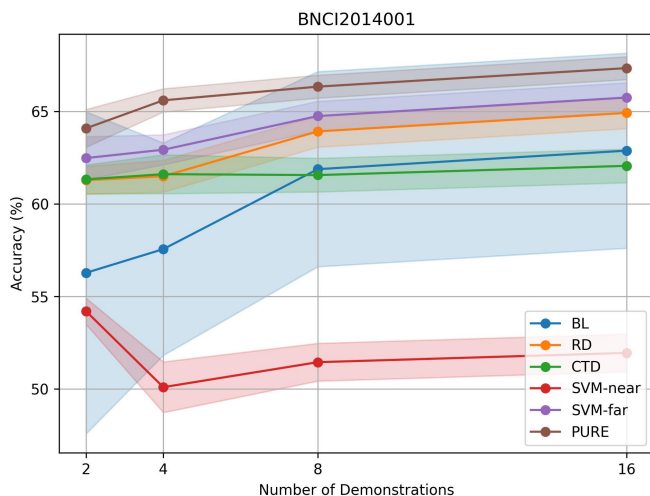
Fig. 3. Performance under different numbers of in-context demonstrations on BNCI2014001 datasets using BL, RD, CTD, SVM-near, SVM-far and PURE methods. The LLM used here is our base model: Qwen-2.5-14b-instruct-1m.
